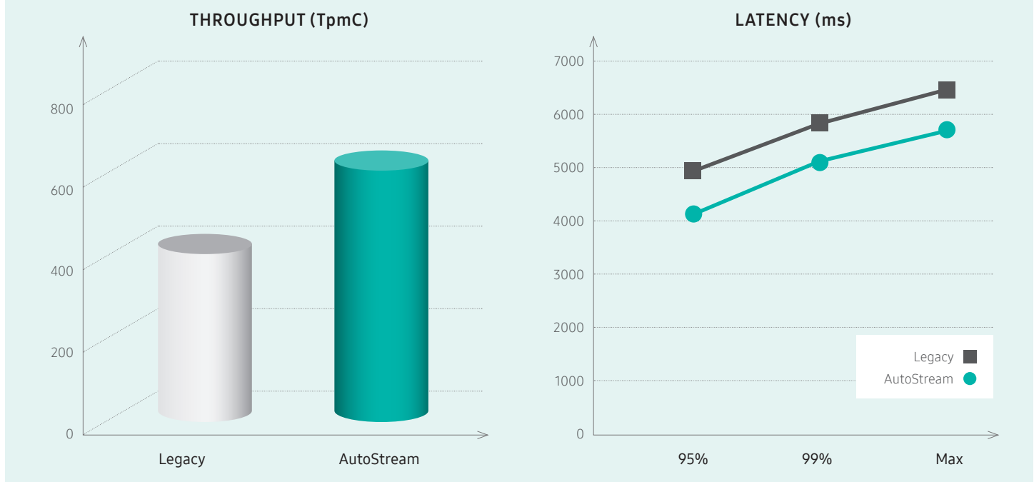
Figure 2.1. MySQL Performance with eight streams (**)
