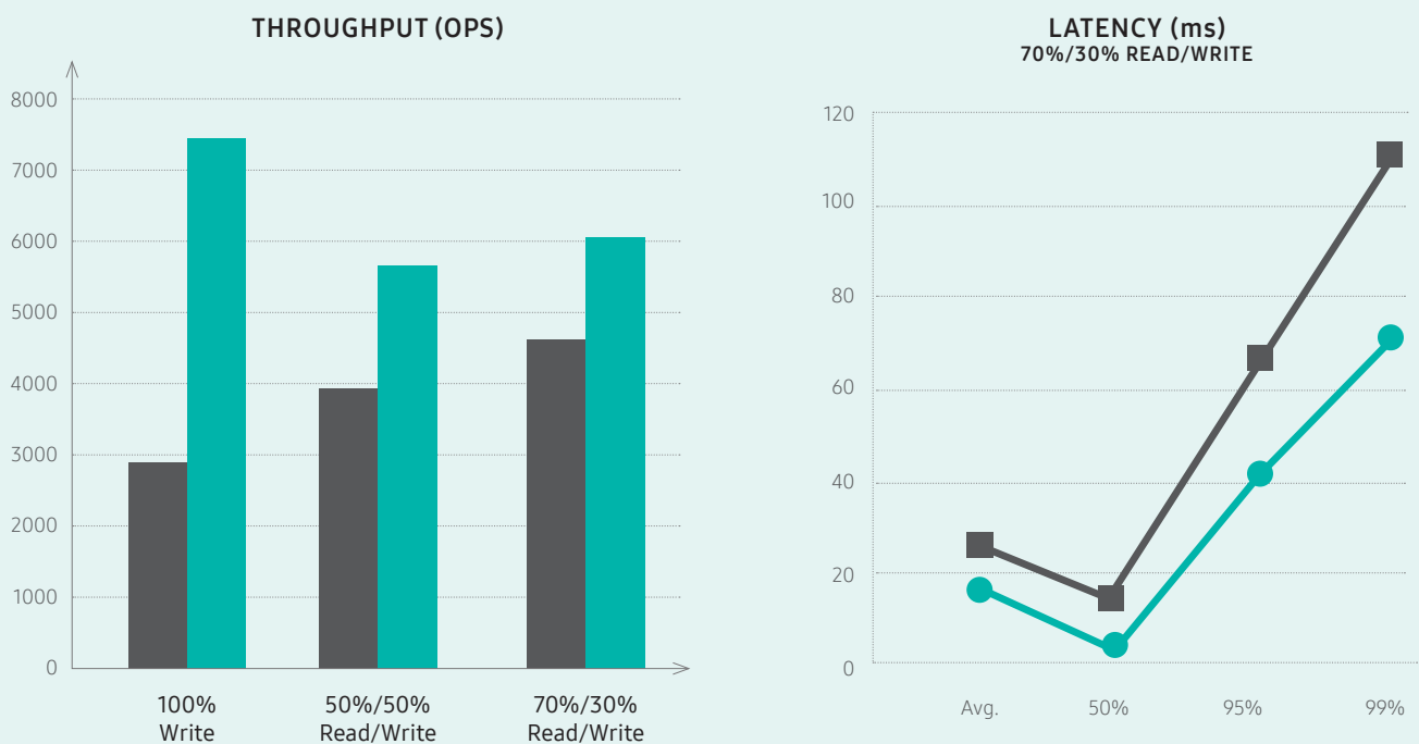
Figure 1. Cassandra Performance with eight streams (*)
